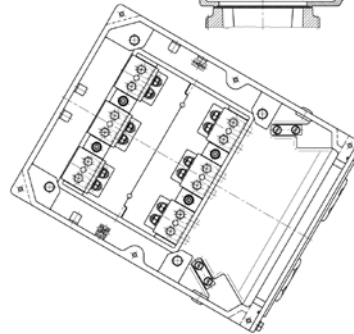
1000 A Ex e IIC, inclined adapter flange
