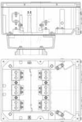
Figure 04G Terminal box 1000 A, straight intermediate flange
