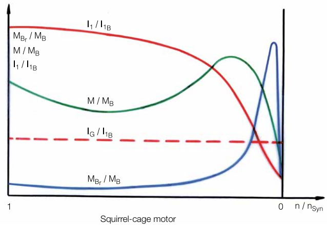
Figure 22: Characteristics for DC braking of a squirrel-cage motor
