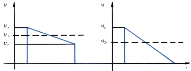
Figure 13: Trapezoidal and triangular reaction torques
