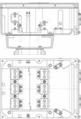
Figure 07G Anschlusskasten 1000 A, Ex eb IIC straight intermediate flange
